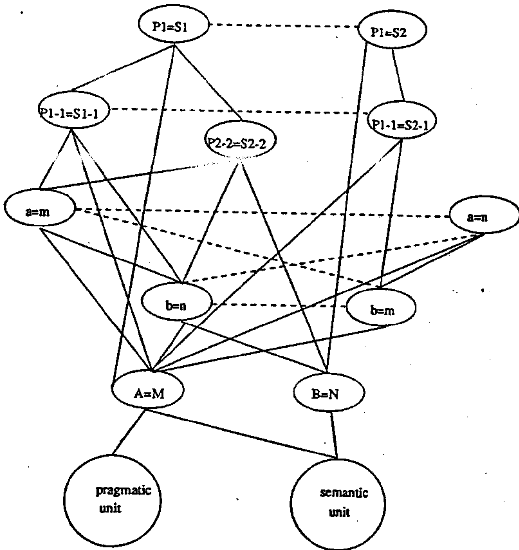
Figure 2. An example of a network constructed by ARCS. Ellipses are units representing possible correspondences. Solid lines indicate excitatory links while dotted lines indicate inhibitory ones.
