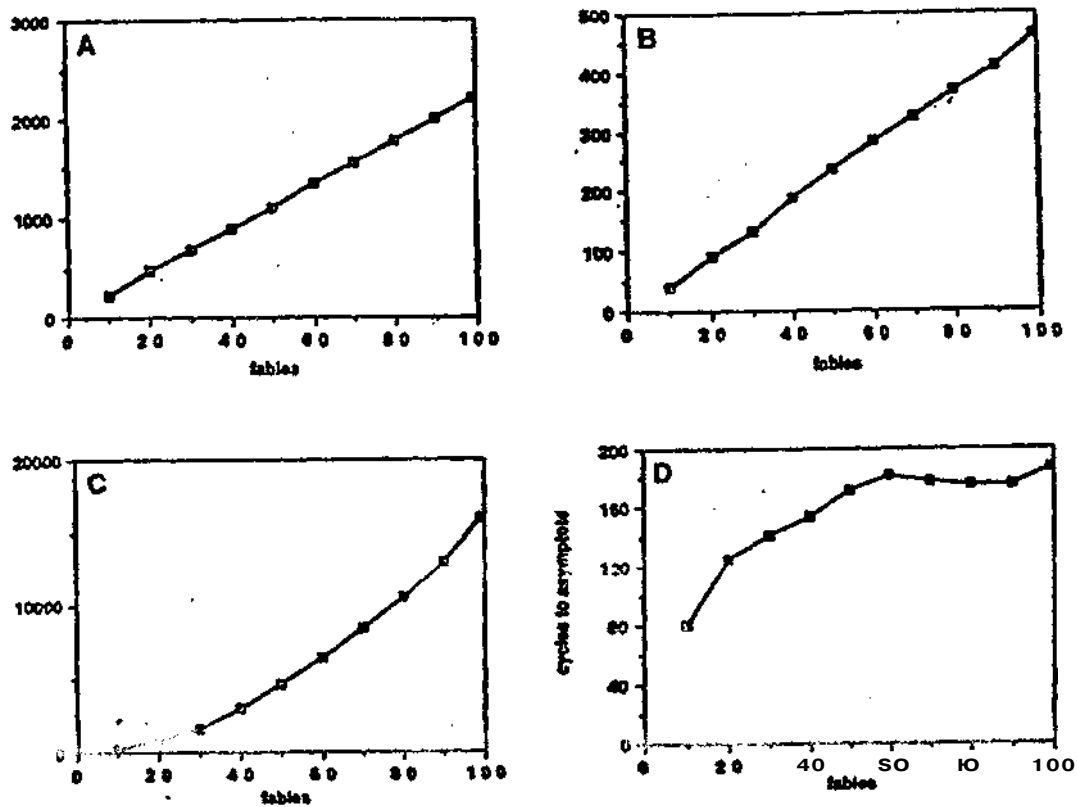
Figure 5. Number of propositions (Panel A), number of units (Panel B), number of links (Panel C), and number of cycles to asymptotic settling (Panel D) as a function of number of fables.
