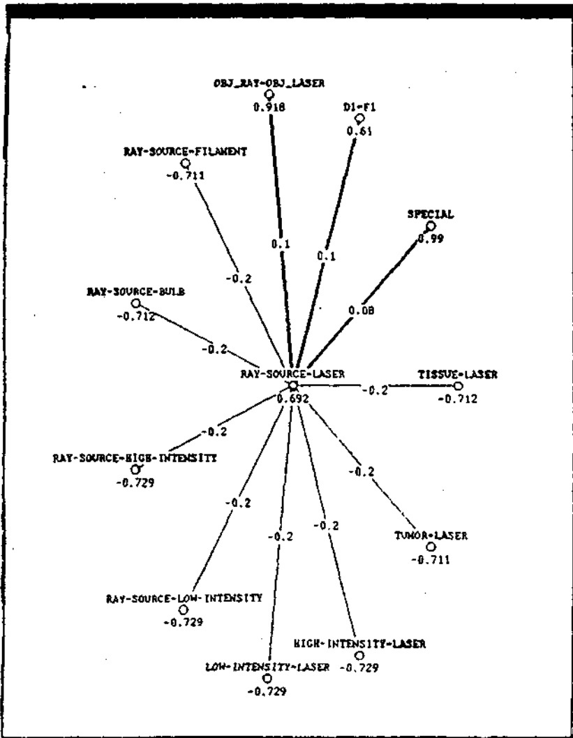
Figure 4. Output of a graphics program running with ACME, showing the subnetwork of excitatory and inhibitory connections to the unit ray-source—loser
