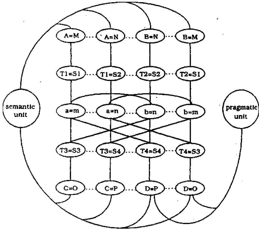
Figur. 2. A schematic example of an ACME mapping network. Numbered capital letters represent proposition identifiers, unnumbered capital letters represent predicates, and lowercase letters represent objects. Solid lines represent excitatory connections and dotted lines represent inhibitory connections. (See text for further explanation.)
