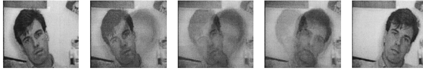
Figure 5: Experiment with the face localist attractor network. Right-tilted images of the 16 different faces are the attractors. Here the initial state is a left-tilted image of one of these faces, and the final state corresponds to the appropriate attractor. The state is shown after every three iterations.
